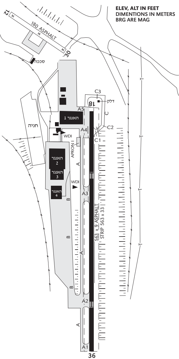
MARKING AIDS RWY 36/18
